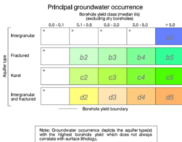
Figure 29: Principal groundwater occurrences in South Africa (Source: Gradient Consulting, 2019).
