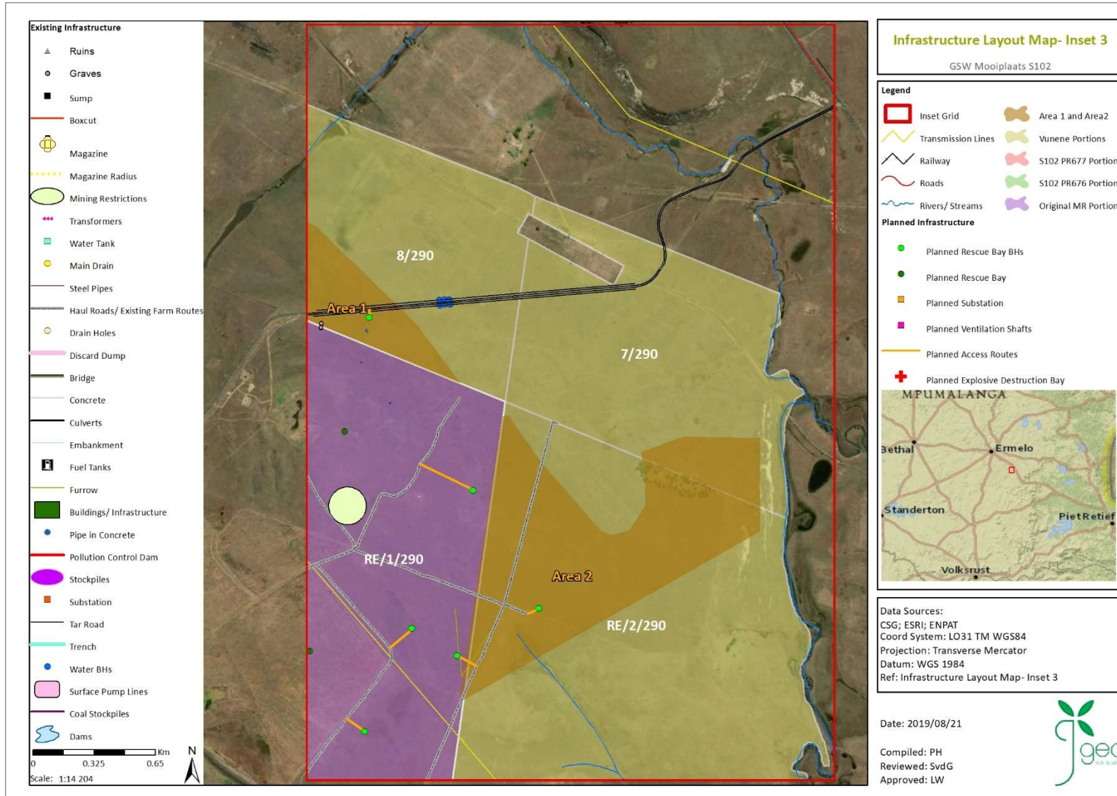
Figure 5: Inset 3 infrastructure layout
