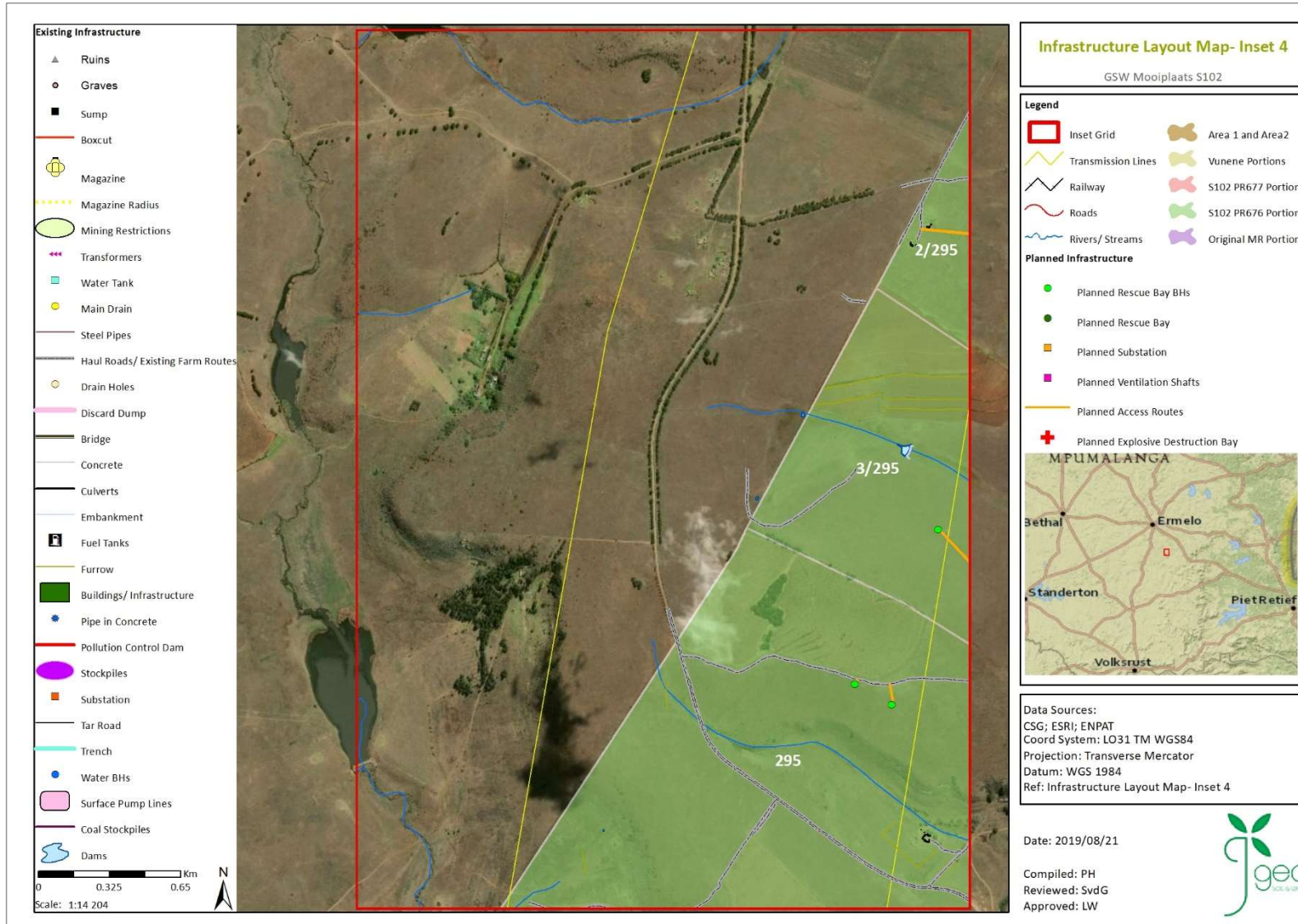
Figure 6: Inset 4 infrastructure layout
