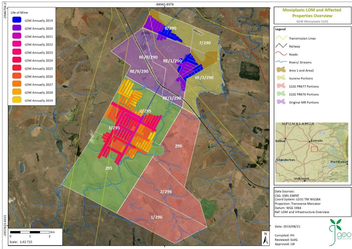
Figure 18: LoM of Mooiplaats Colliery indicating the location of the underground resources
