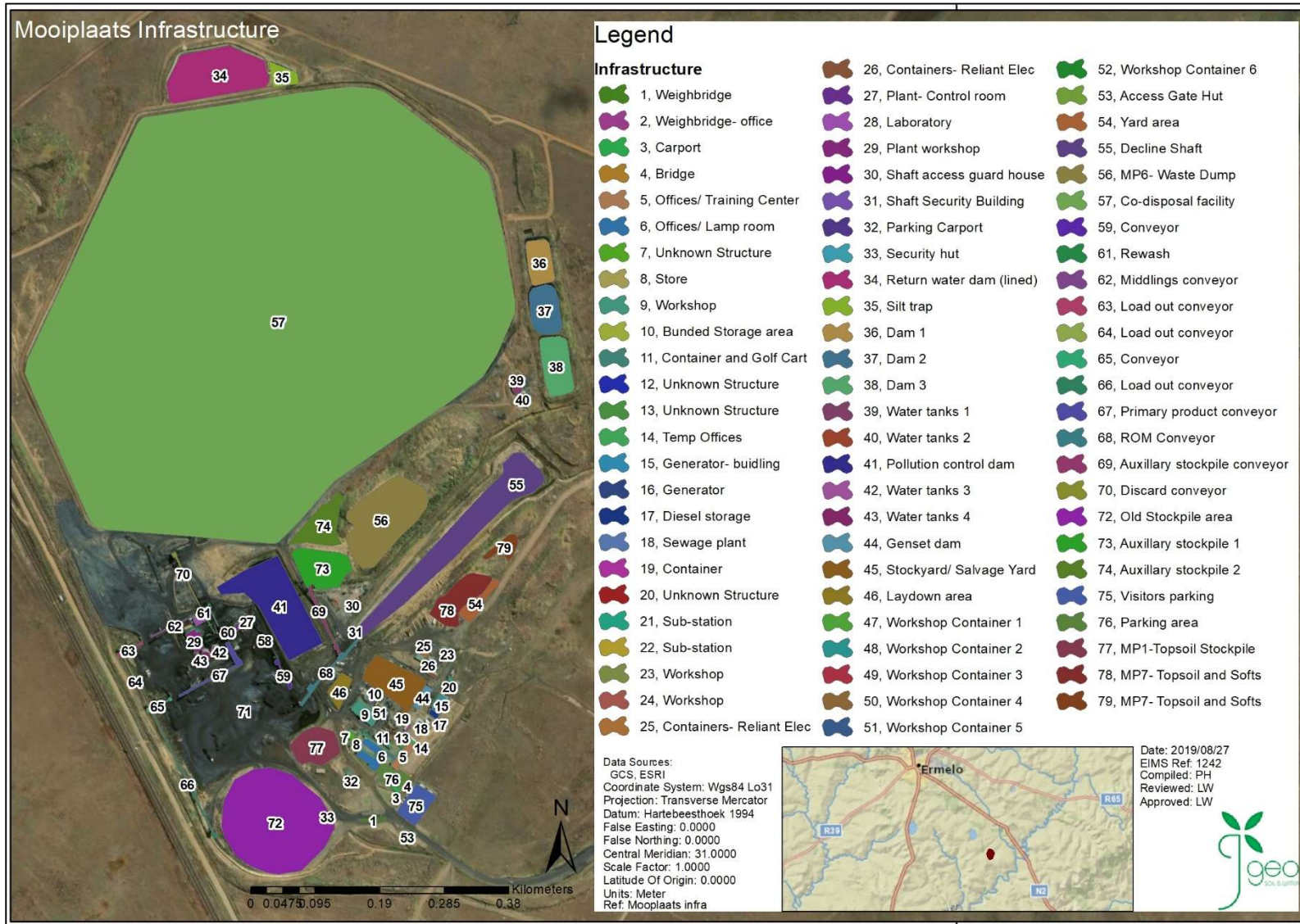
Figure 13: Existing infrastructure layout at the Mooiplaats Colliery
