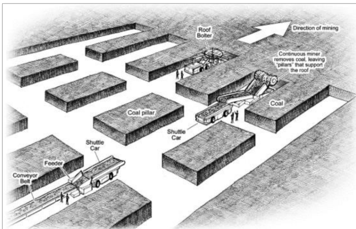
Figure 20: Illustration of bord and pillar mining
