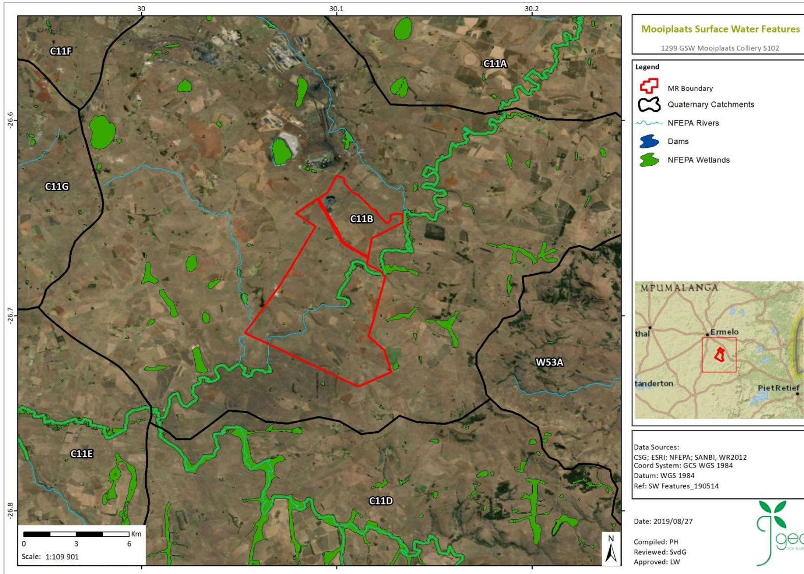
Figure 27: Mooiplaats Colliery surface water features
