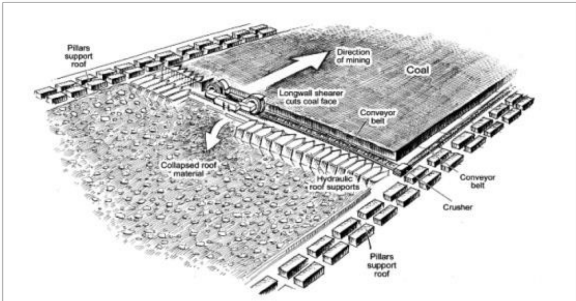
Figure 19: Illustration of long wall mining
